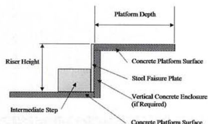
Stadium Platform Section Diagram is intended for illustration purposes only
